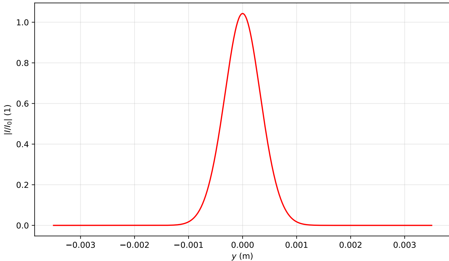
Intensity profile I(x=0, y, z=0.239)/I_0 , P_{in}=1.0P_{cr} , artificial time
